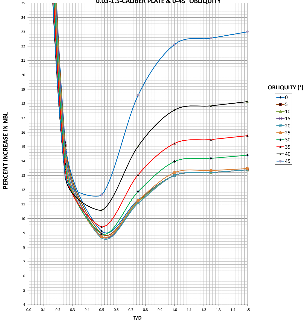
5% WINDSCREEN + 5% HOOD EFFECT ON NBL DETAILS: 0.03-1.5-CALIBER PLATE & 0-45° OBLIQUITY
