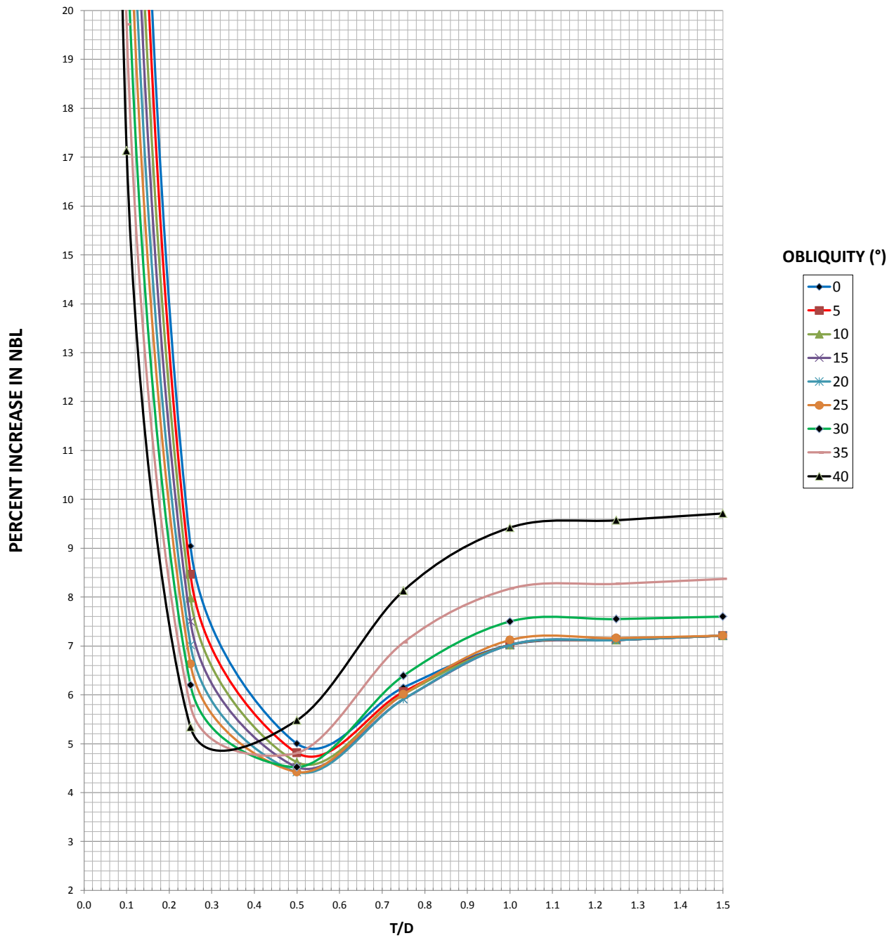
5% HOOD EFFECT ON NBL DETAILS: 0.001-1.5-CALIBER PLATE & 0-40° OBLIQUITY
