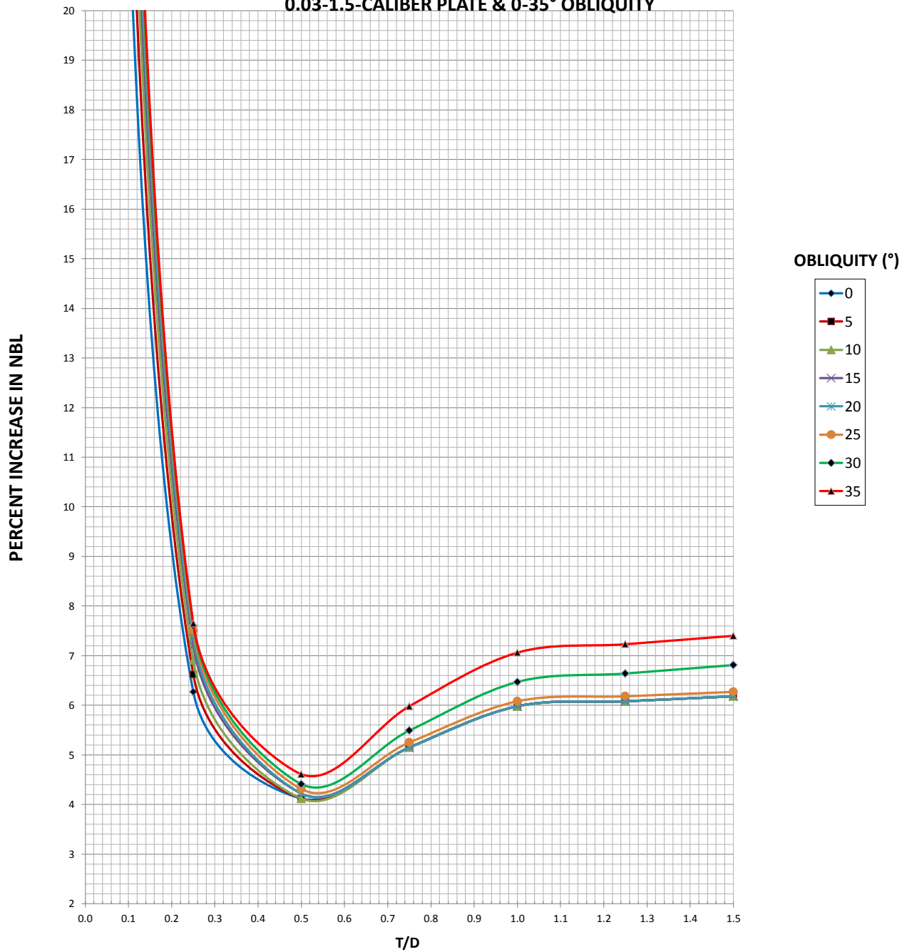
5% WINDSCREEN EFFECT ON NBL DETAILS: 0.03-1.5-CALIBER PLATE & 0-35° OBLIQUITY
